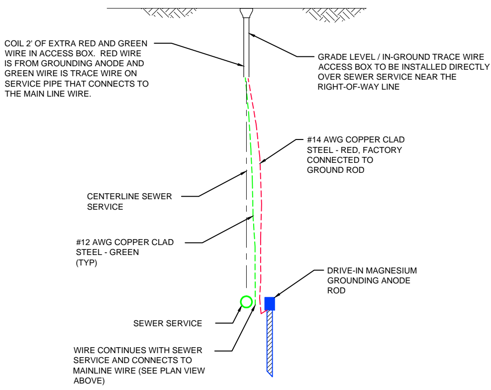
SEWER SERVICE - SECTION VIEW NO SCALE
